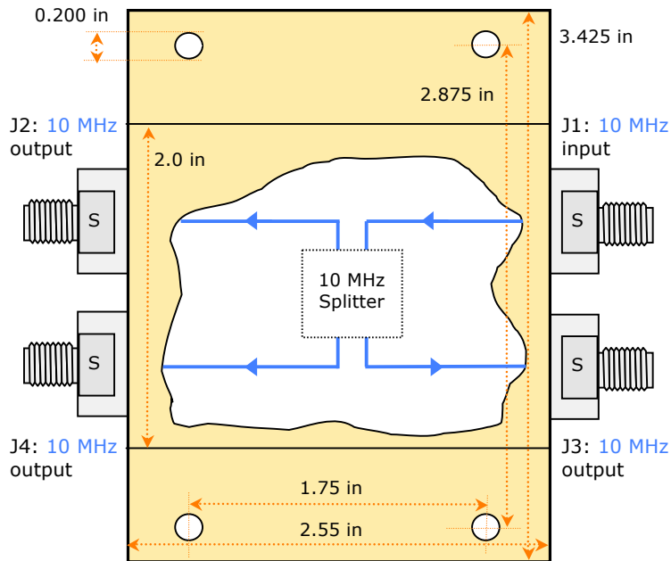
Orbital 10 MHz Splitter Mechanical Dimensions + Functional Block Diagram Viewed from top
